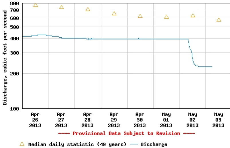
USGS 01425000 WEST BR DELAWARE RIVER AT STILESVILLE NY
